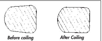
Modified trapezoidal cross section of rectangular wire springs changes to a "D" cross section during coiling.
